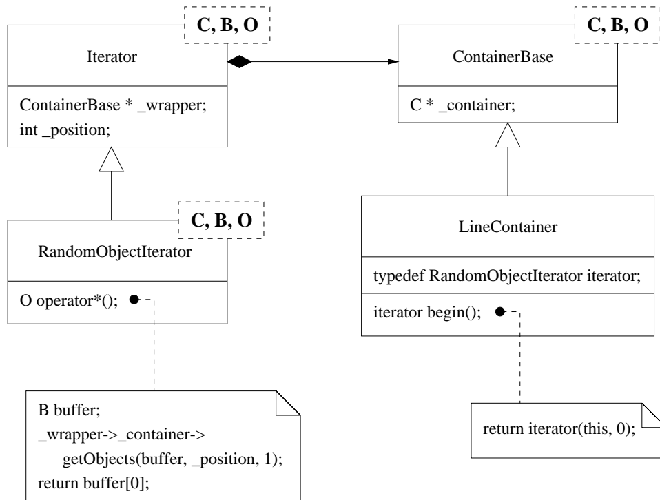
Figure 4: UML class diagram of relationship between LineContainer and RandomObjectIterator objects. Containers may retrieve groups of data objects and cache them (not shown) to reduce the number of network requests. C is Container Type ; B is Buffer Type ; O is Object Type .
